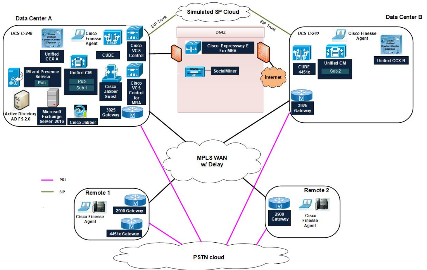
Figure 1: Collaboration Systems Release 12.7: Unified CCX Test Architecture
