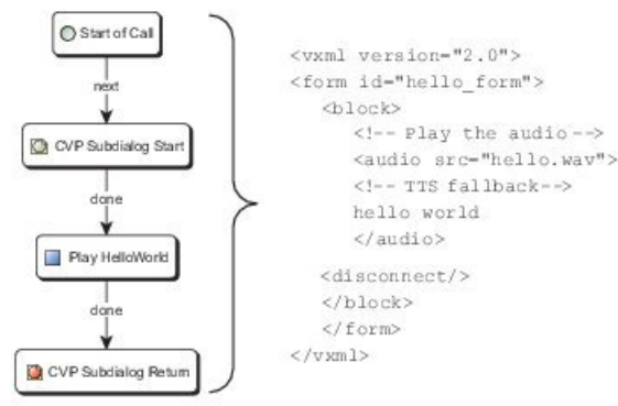
Figure 4: Call Studio Generates the Code for You
