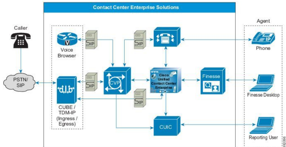
Figure 24: CUSP in a Contact Center Enterprise Solution
