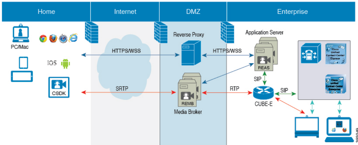
Figure 22: Remote Expert Mobile Deployment
