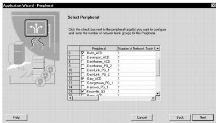
Figure 26: Application Wizard—Peripheral
