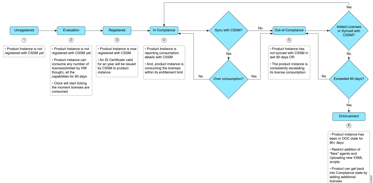
Figure 7: License States
