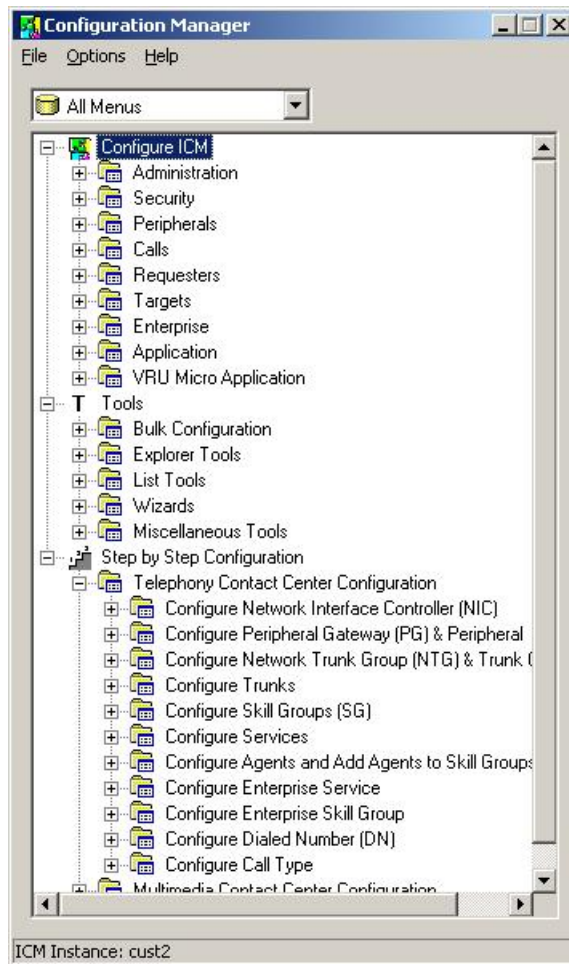
Figure 10: Configuration Manager
