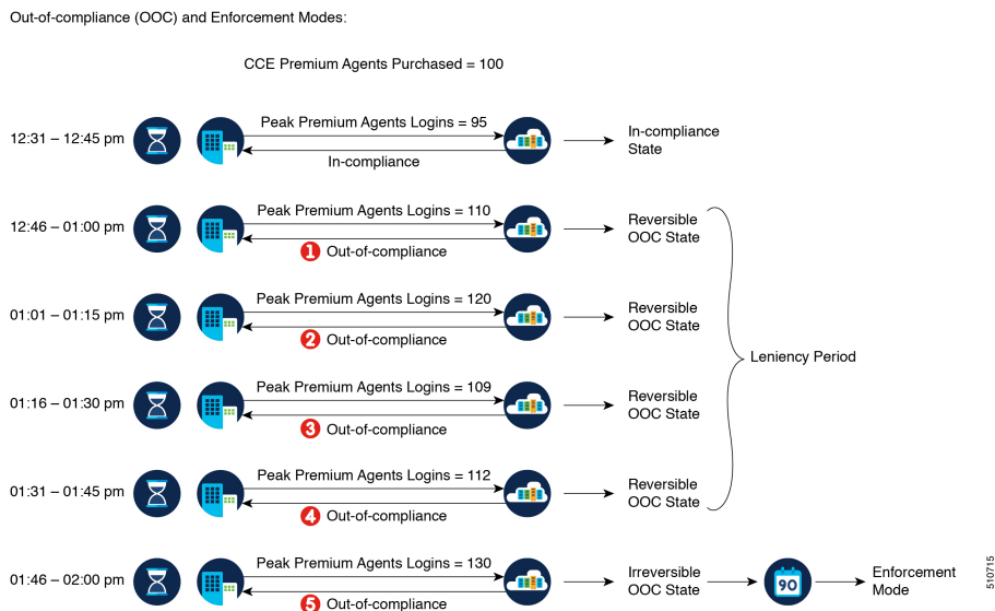
Figure 8: License Computation
