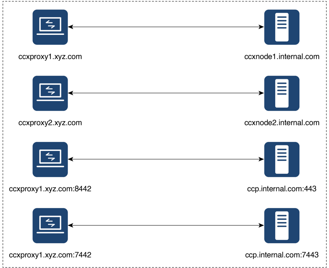
Figure 1: Hostname Mapping Example
