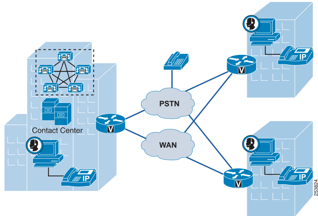
Figure 22-4 Multisite Contact Center with Centralized Call Processing
