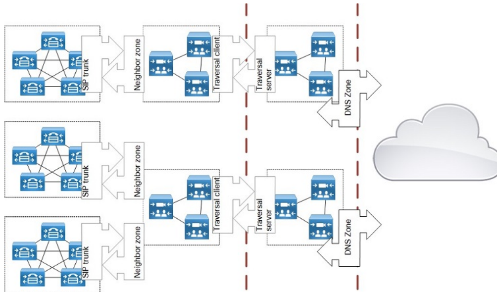
Figure 1: Sample Deployment Showing Multiple Clusters, Trunks, and Zones
