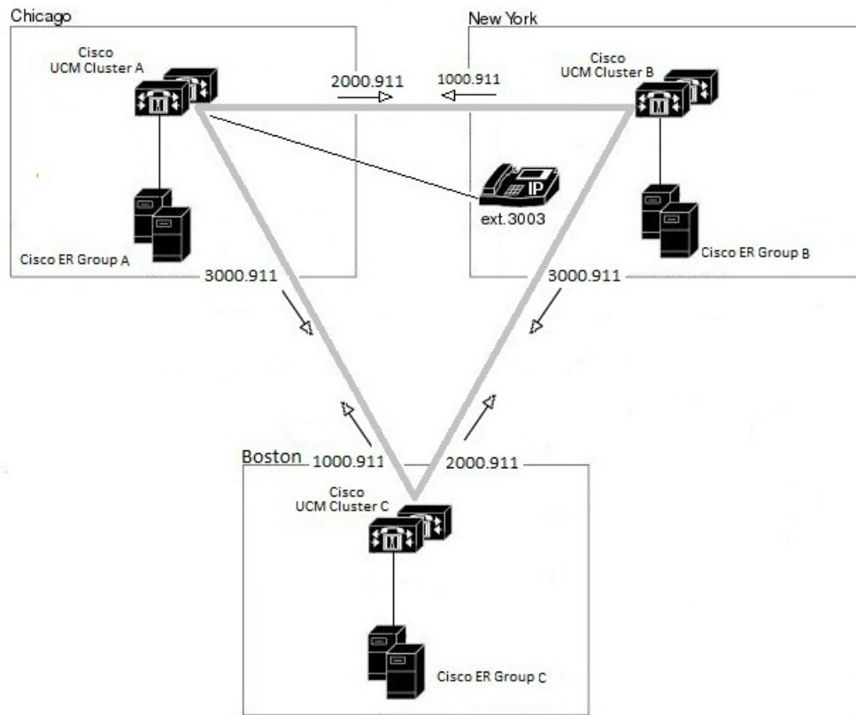
Figure 1: Understanding Inter-Cisco Emergency Responder Group Route Patterns
