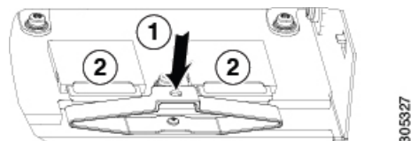
Figure 4: SD Card Slots
