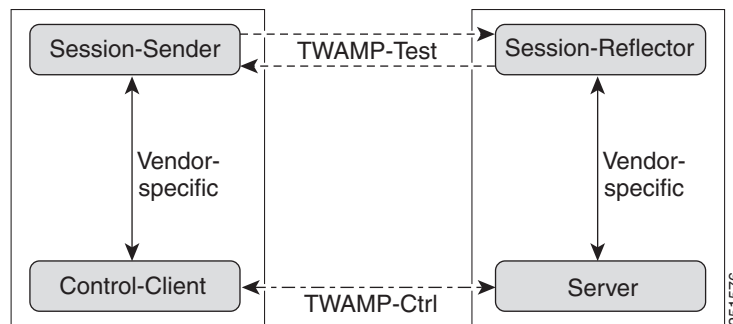
Figure 41-4 TWAMP Architecture
