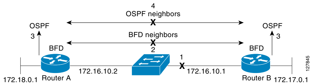
Figure 33-7 Breaking an OSPF Neighbor Relationship
