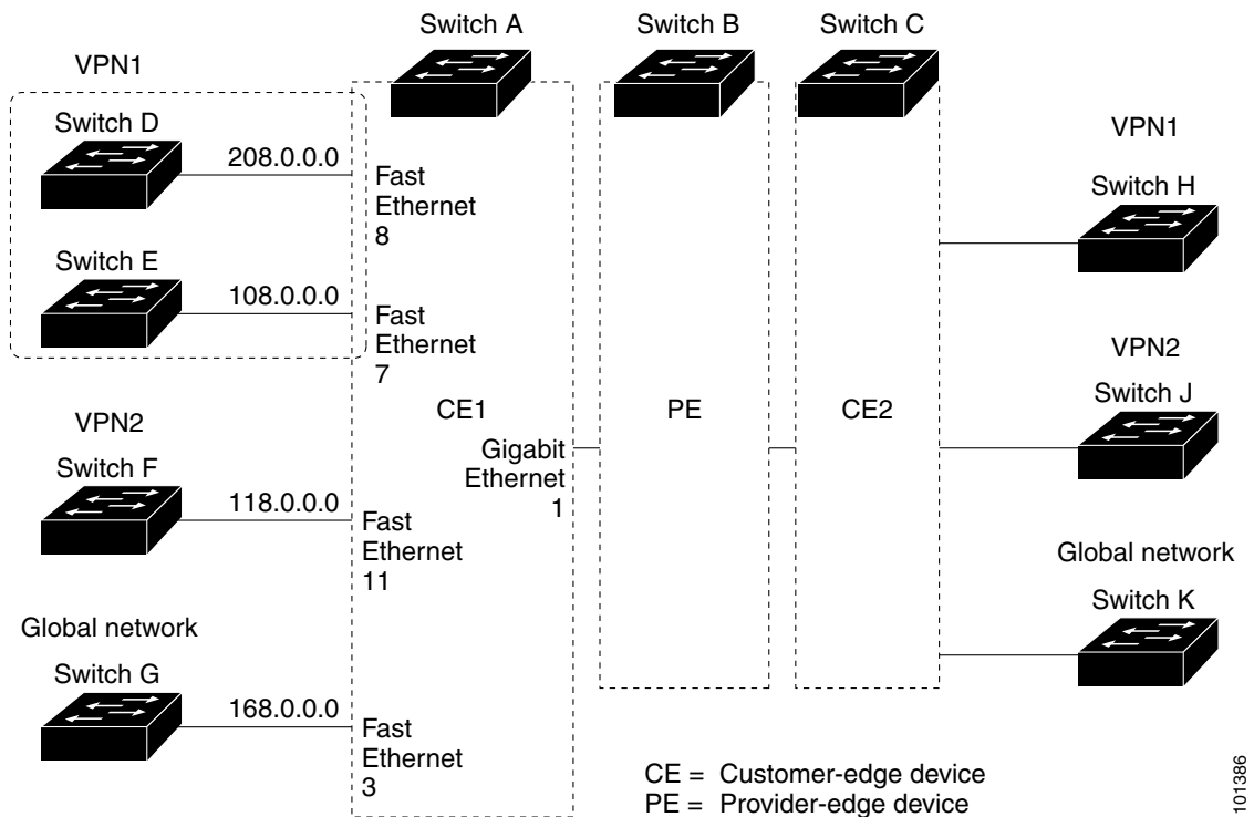
Figure 33-9 Multi-VRF CE Configuration Example
