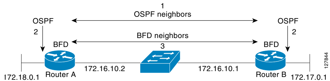
Figure 33-6 Establishing a BFD Session
