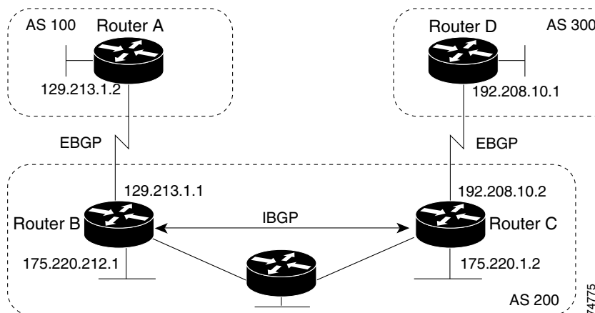
Figure 33-5 EBGP, IBGP, and Multiple Autonomous Systems
