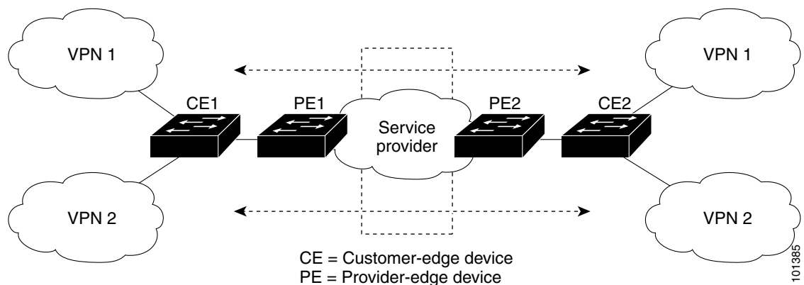
Figure 33-8 Switches Acting as Multiple Virtual CEs
