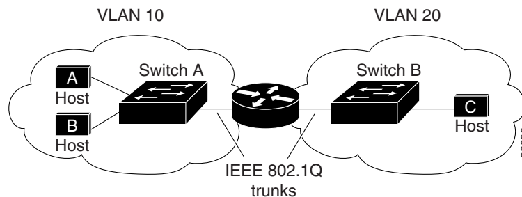
Figure 33-1 Routing Topology Example
