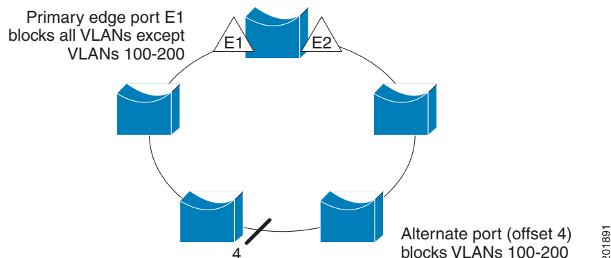
Figure 22-5 Example of VLAN Blocking
