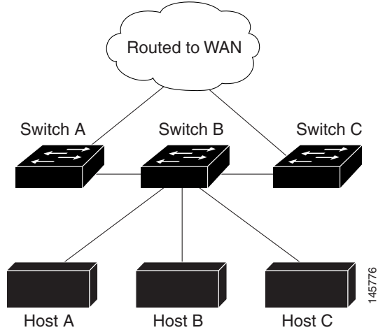
Figure 40-4 EIGRP Stub Router Configuration
