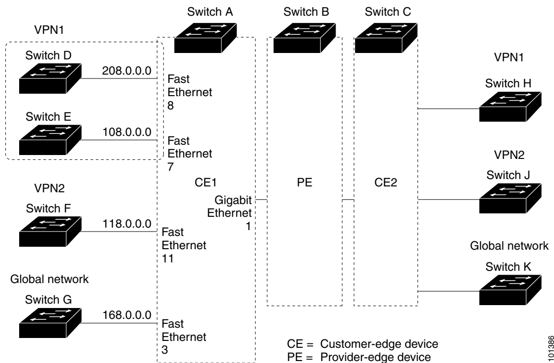
Figure 40-7 Multi-VRF CE Configuration Example
