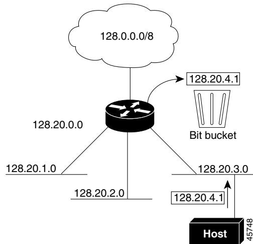
Figure 40-3 No IP Classless Routing
