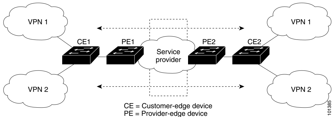
Figure 40-6 Switches Acting as Multiple Virtual CEs
