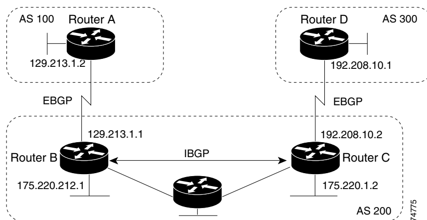
Figure 40-5 EBGP, IBGP, and Multiple Autonomous Systems
