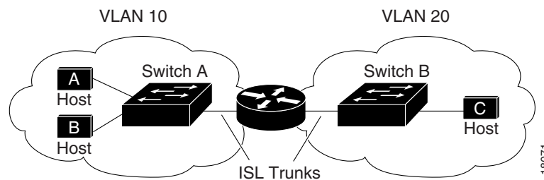
Figure 40-1 Routing Topology Example
