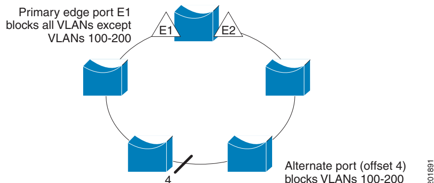
Figure 24-5 Example of VLAN Blocking
