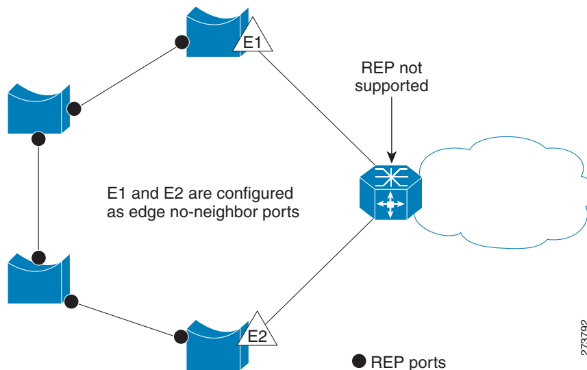
Figure 21-3 Edge No-Neighbor Ports
