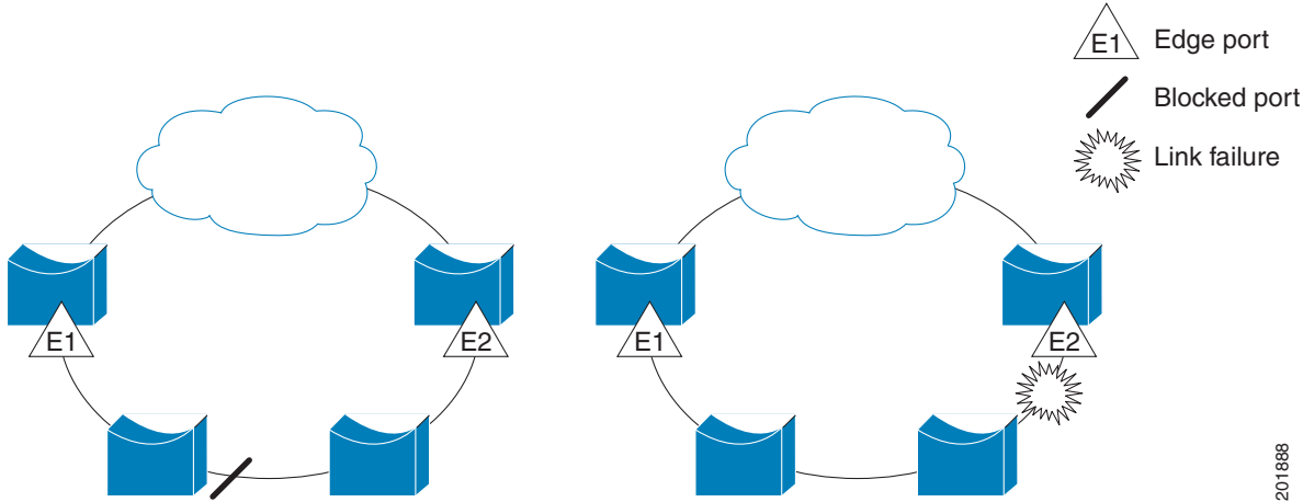
Figure 21-1 REP Open Segments
