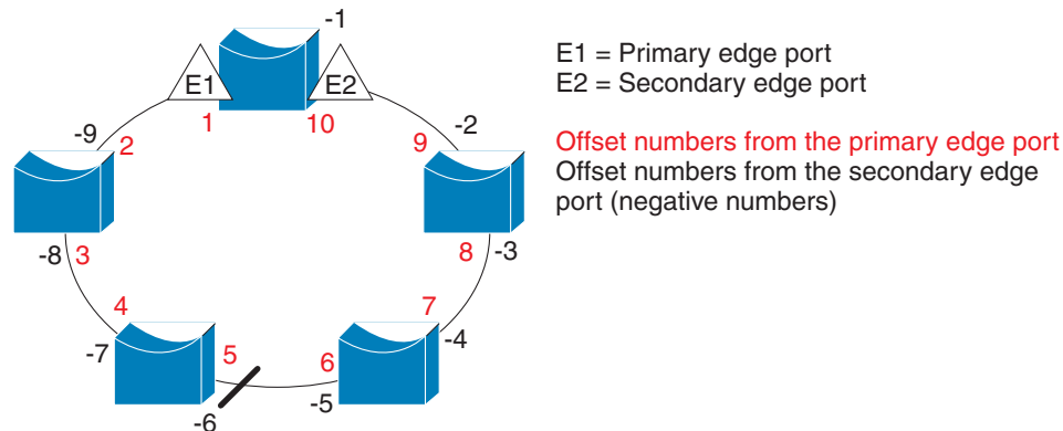
Figure 21-4 Neighbor Offset Numbers in a Segment
