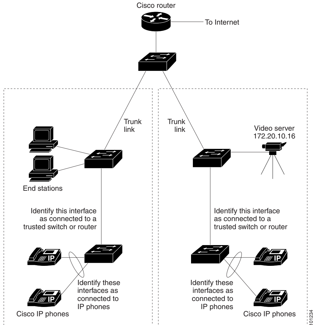
Figure 33-10 Auto-QoS Configuration Example Network
