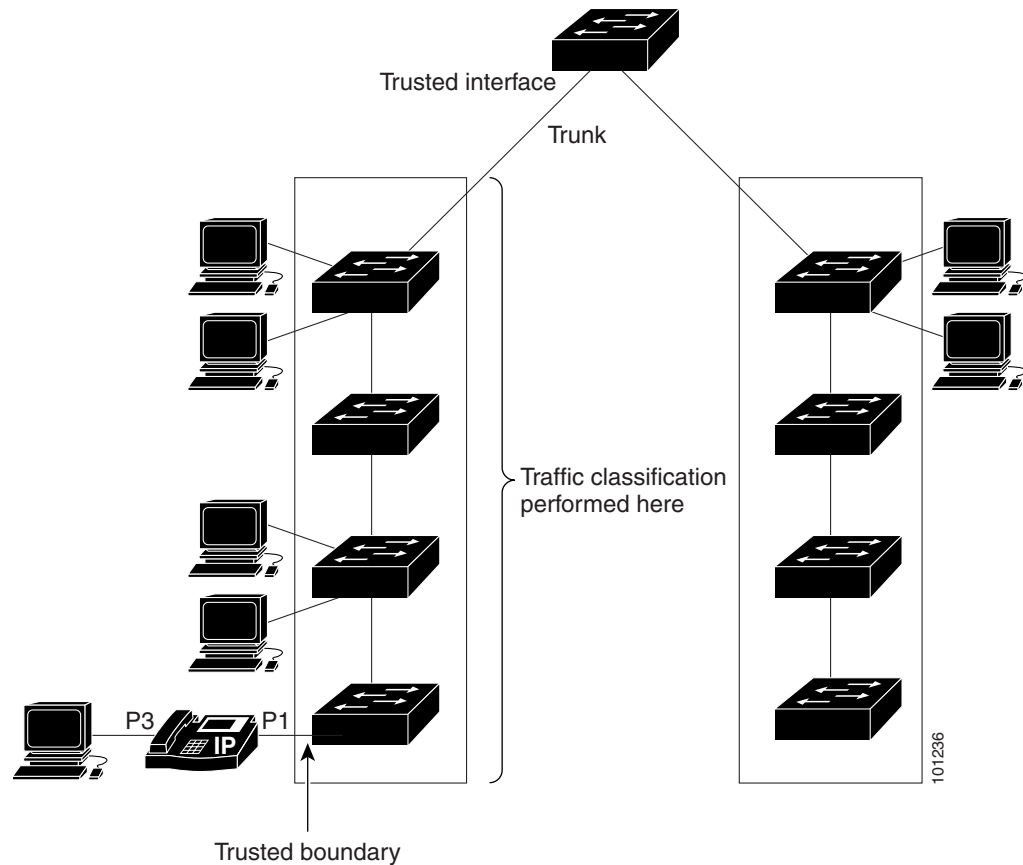
Figure 33-11 Port Trusted States within the QoS Domain
