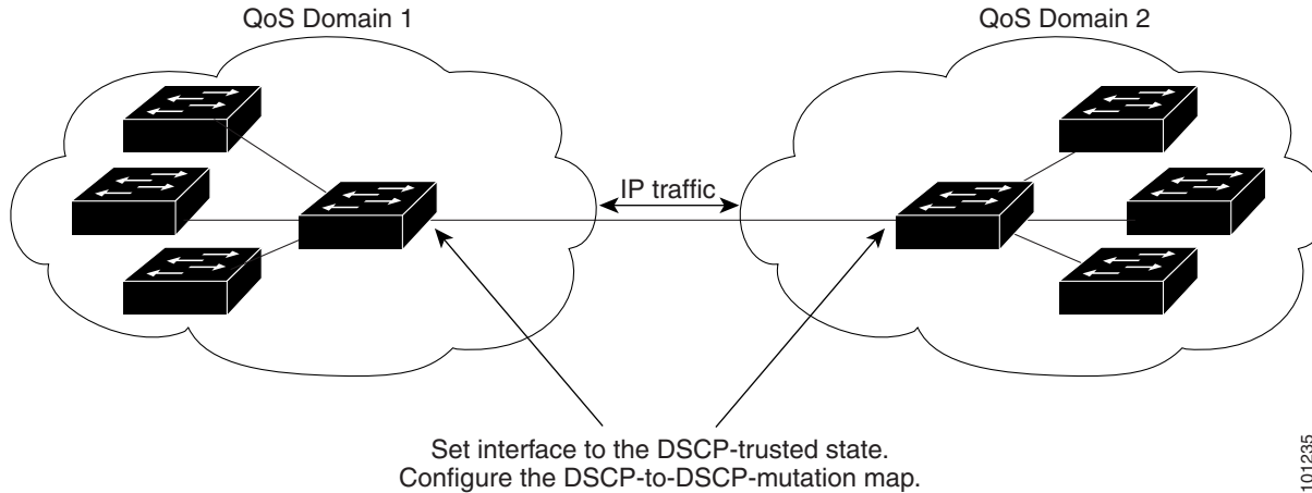
Figure 33-12 DSCP-Trusted State on a Port Bordering Another QoS Domain
