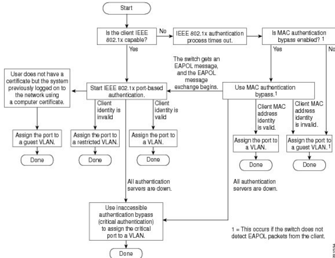
Figure 21: Authentication Flowchart
