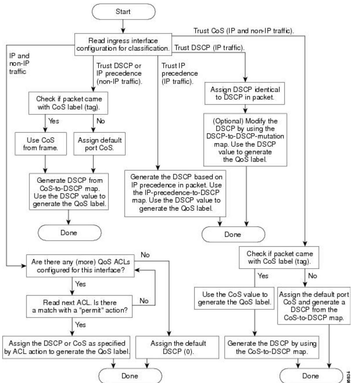
Figure 3: Classification Flowchart
