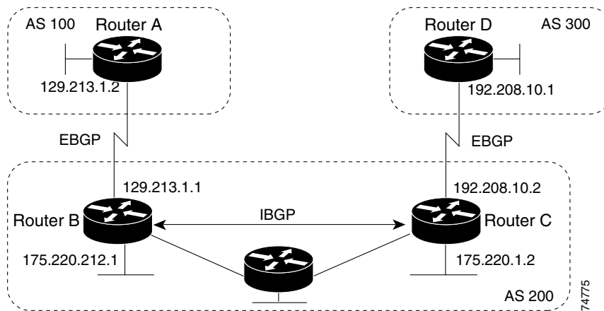
Figure 31-4 EBGP, IBGP, and Multiple Autonomous Systems
