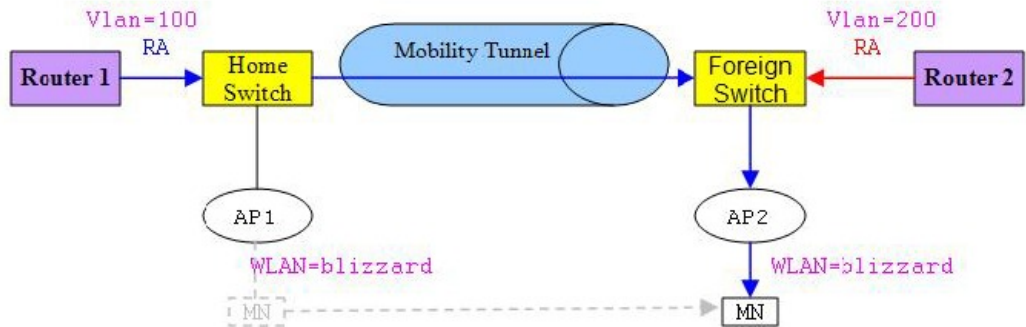
Figure 2: Roaming Client Receives Valid RA from Router 1
