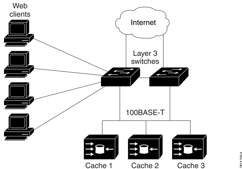
Figure 40-1 Cisco Cache Engine and WCCP Network Configuration
