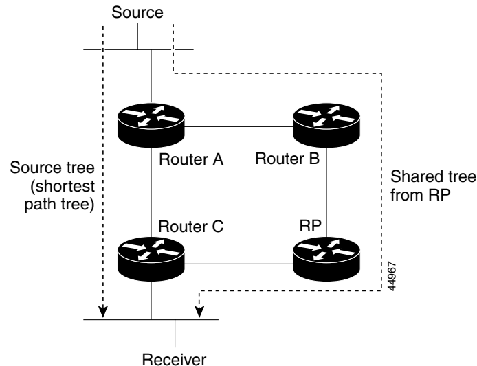
Figure 35-4 Shared Tree and Source Tree (Shortest-Path Tree)
