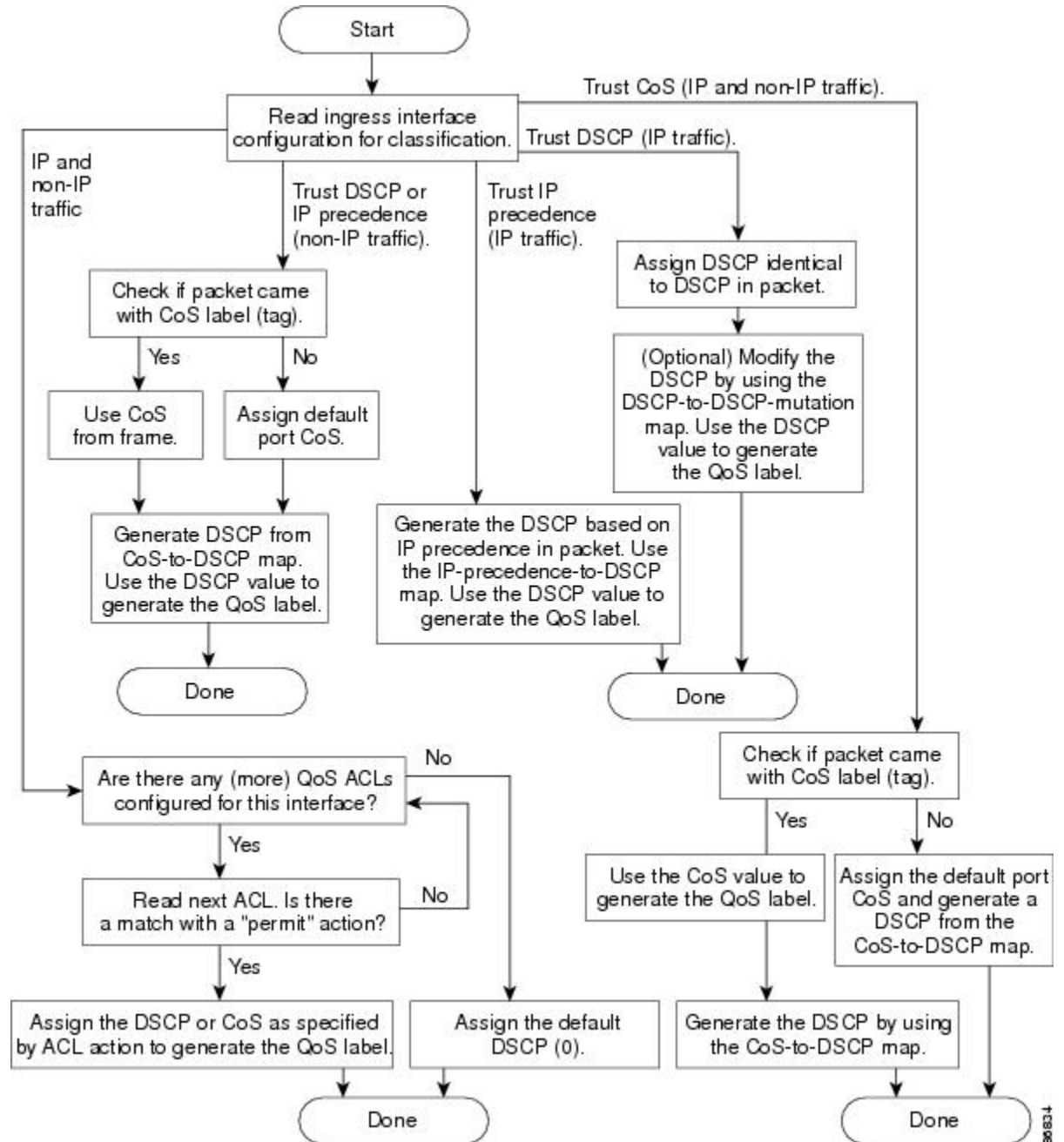
Figure 3: Classification Flowchart
