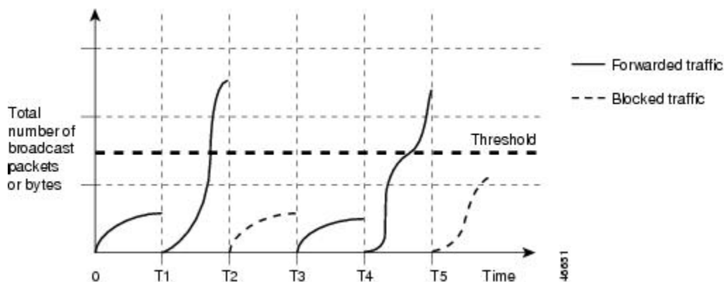
Figure 1: Broadcast Storm Control Example
