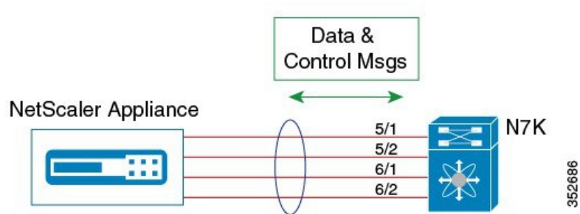
Figure 1: Direct Connect Mode for the Appliance and a Standalone Switch
