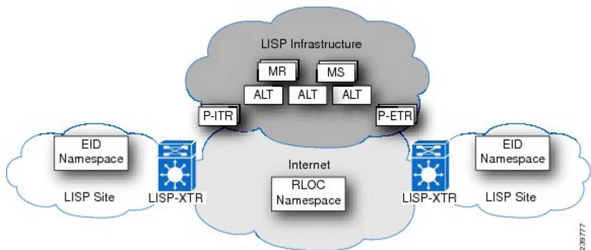
Figure 1: Cisco NX-OS LISP Deployment Environment
