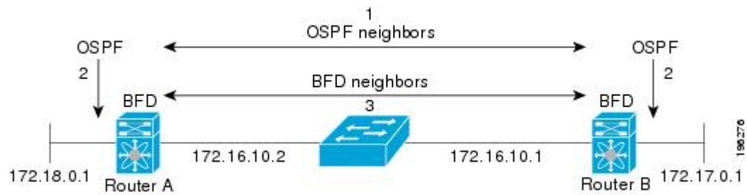
Figure 1: Establishing a BFD Neighbor Relationship
