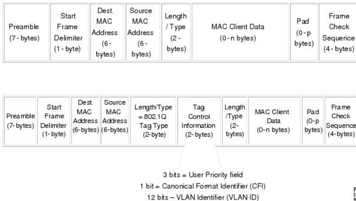
Figure 2: Header Without and With 802.1Q Tag Included
