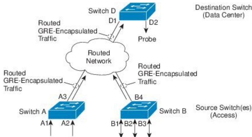
Figure 1: ERSPAN Configuration
