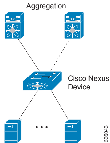
Figure 2 Access Switch Topology
