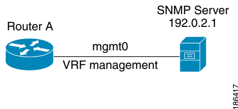
Figure 11-2 Service VRF Reachability
