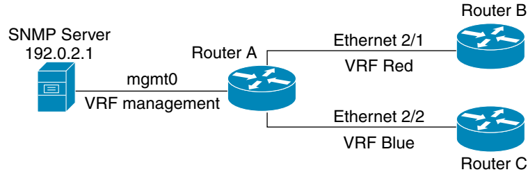
Figure 11-4 Service VRF Reachability Filtering
