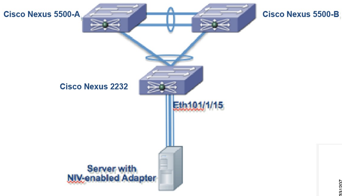
Figure 1: Cisco Nexus Adapter FEX Dual-Homed Topology
