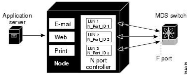
Figure 2: NPIV Example
