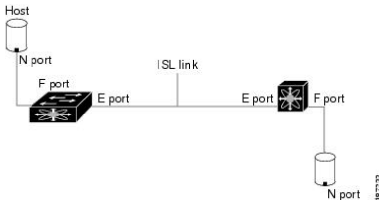
Figure 1: Switch Port Modes
