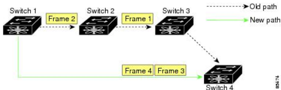
Figure 4: Route Change Delivery
