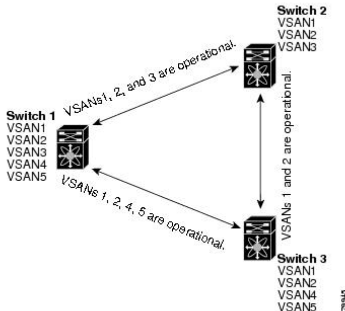
Figure 3: Default Allowed-Active VSAN Configuration
