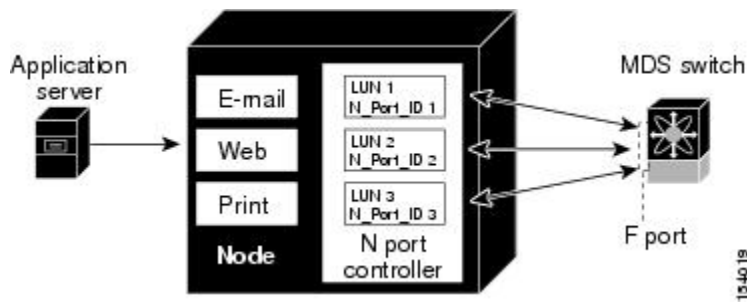
Figure 1: NPIV Example
