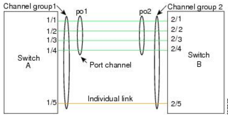
Figure 1: Individual Links Combined into an EtherChannel
