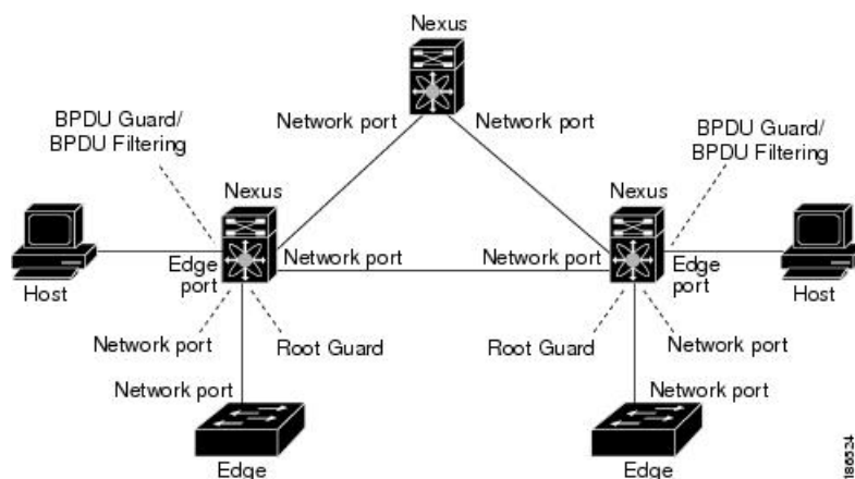
Figure 5: Network with STP Extensions Correctly Deployed
