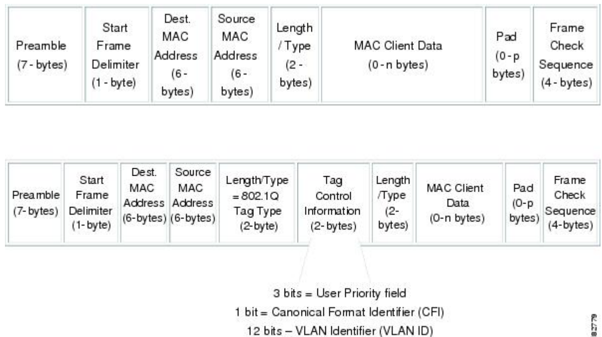
Figure 1: Header without and with 802.1Q Tag Included
