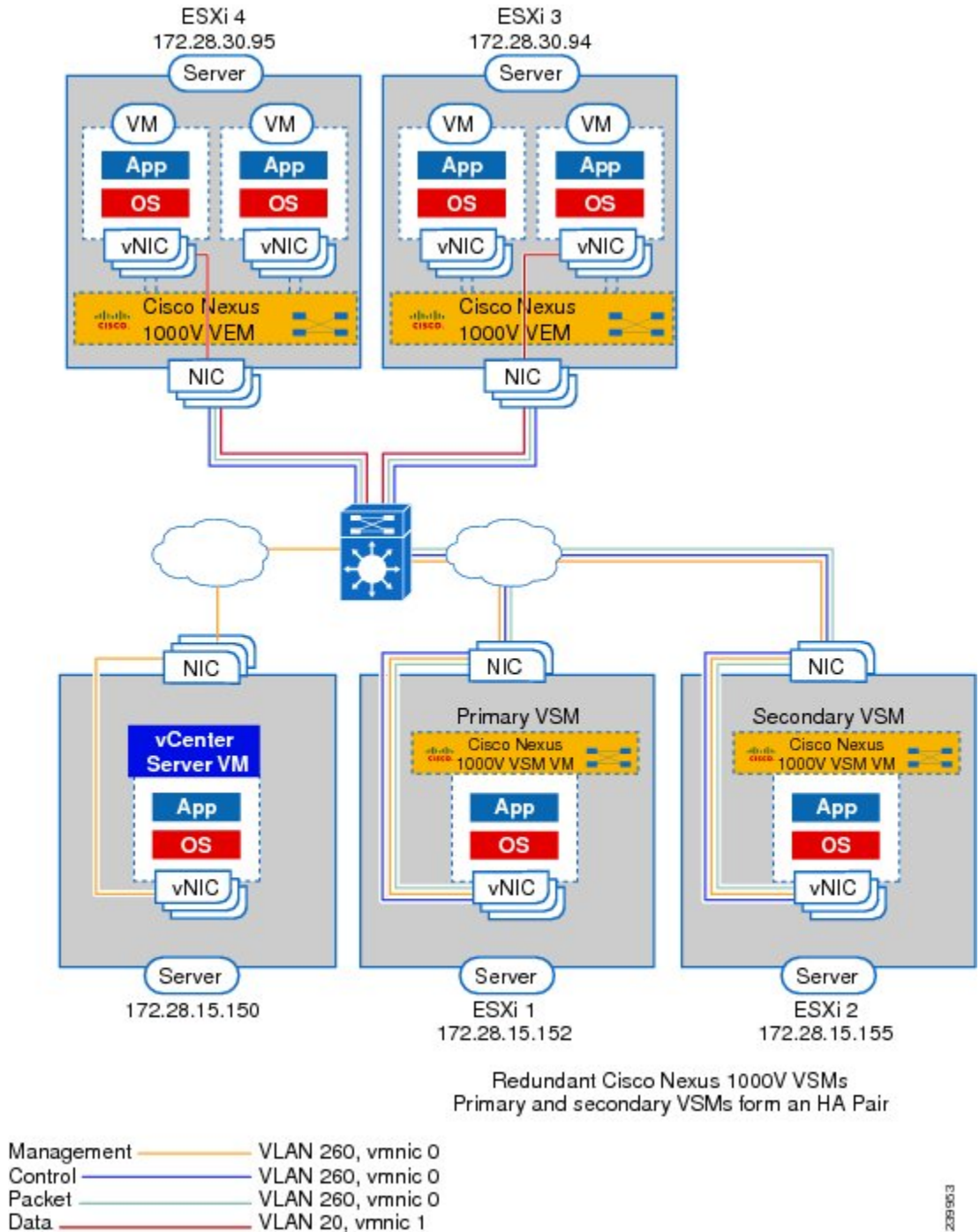
Figure 4: Layer 2 Control Mode Topology Diagram
