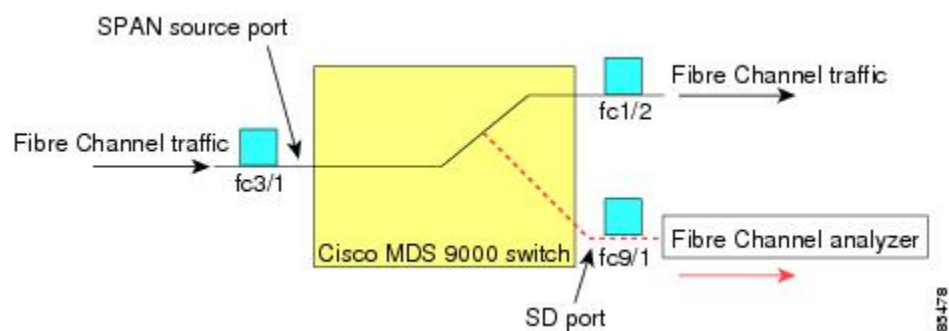
Figure 1: SPAN Transmission
