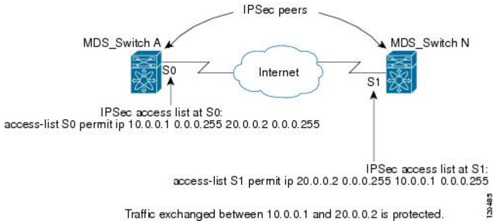
Figure 5: IPsec Processing of Crypto IPv4-ACLs
