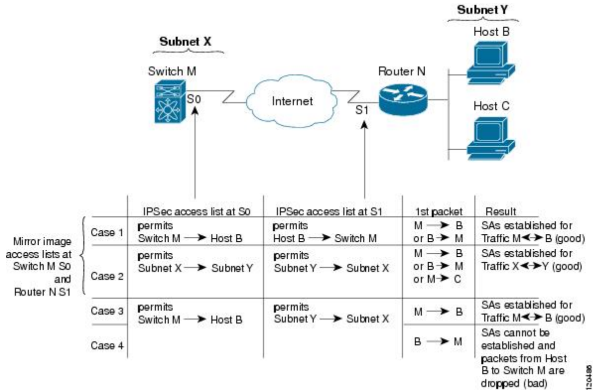
Figure 6: IPsec Processing of Mirror Image Configuration
