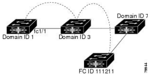
Figure 4: Fibre Channel Routes
