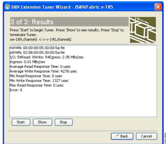
Figure 3-6 Results Dialog Box
