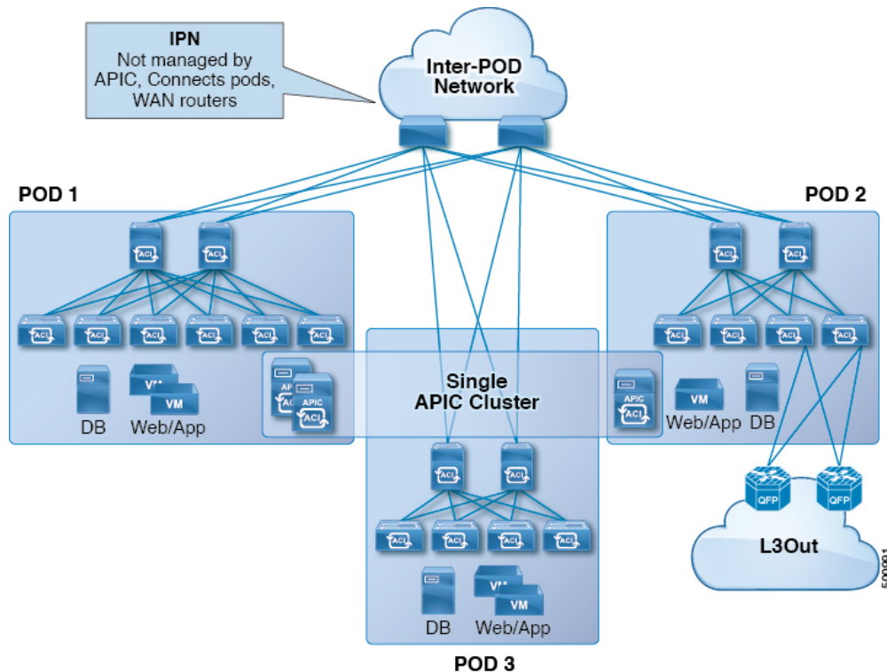
Figure 74: Multipod Overview
