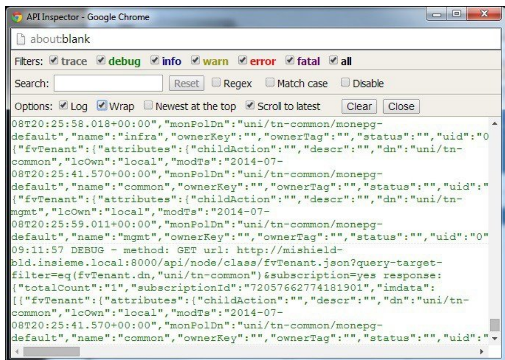
Figure 109: API Inspector
