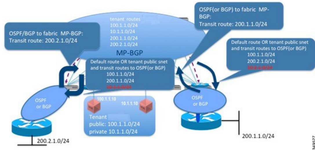
Figure 85: Route Redistribution
