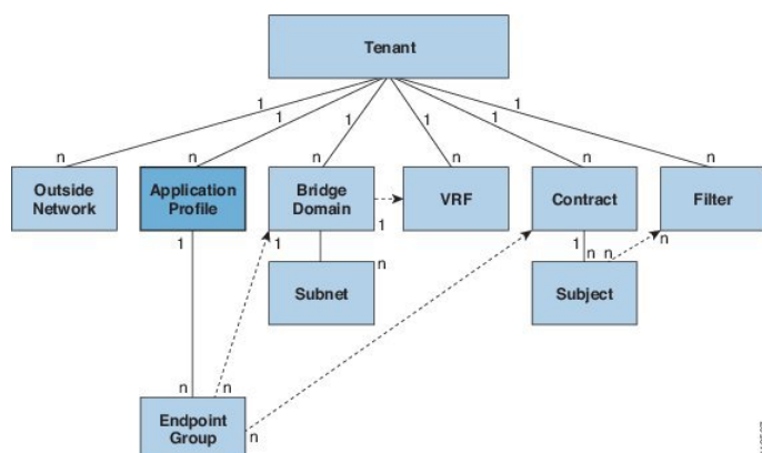
Figure 8: Application Profiles
