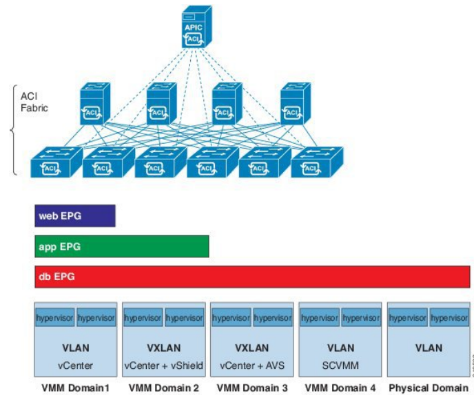
Figure 94: Multiple VMM Domains and Scaling of EPGs in the Fabric
