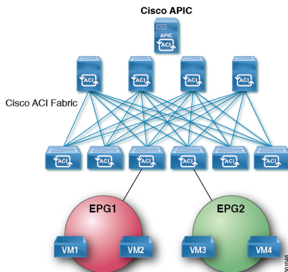
Figure 49: VM1 to VM2 Communication is Desired.
