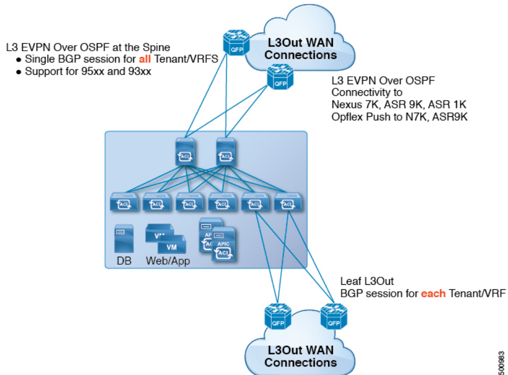
Figure 73: Cisco ACI GOLF Topology
