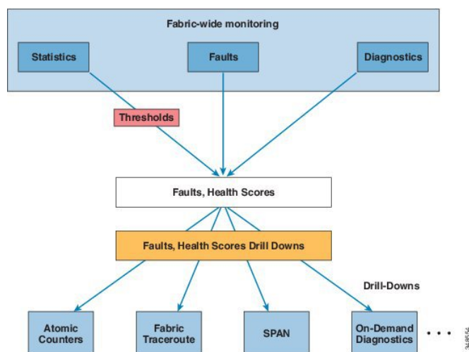
Figure 128: Troubleshooting
