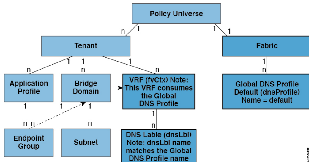
Figure 58: DNS
