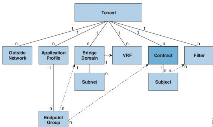
Figure 15: Contracts
