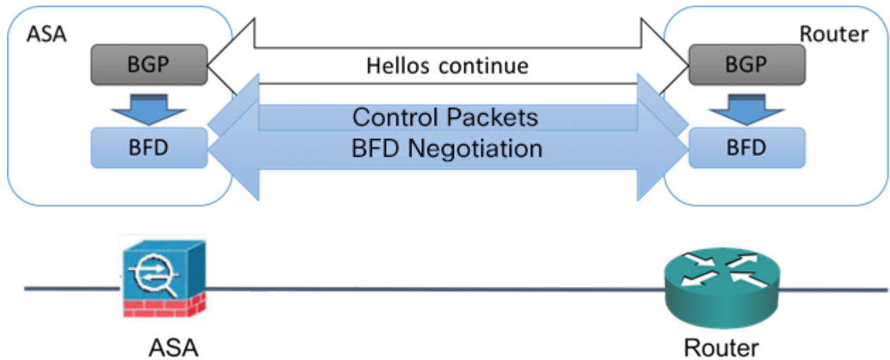
Figure 45: BFD Session Established
