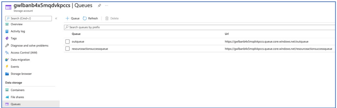
Figure 13: Outqueue
