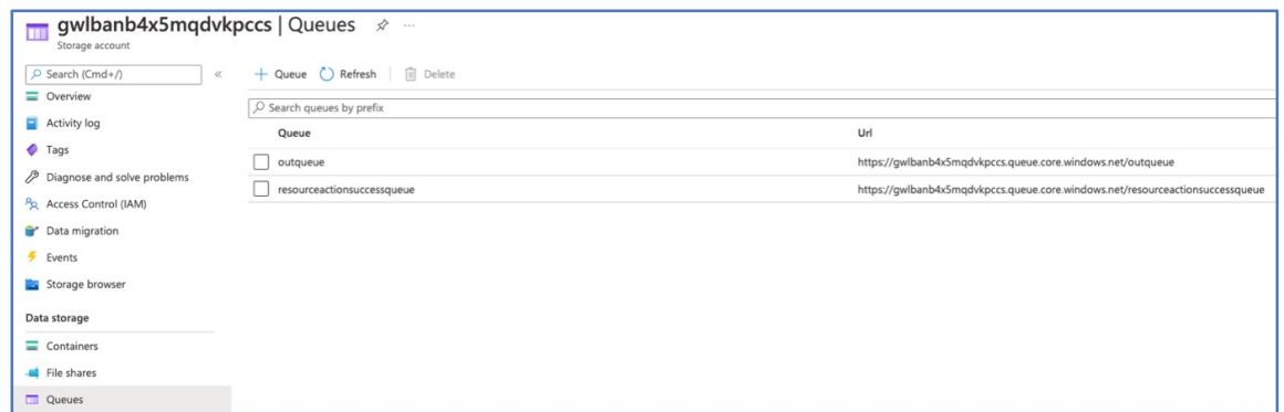
Figure 13: Outqueue
