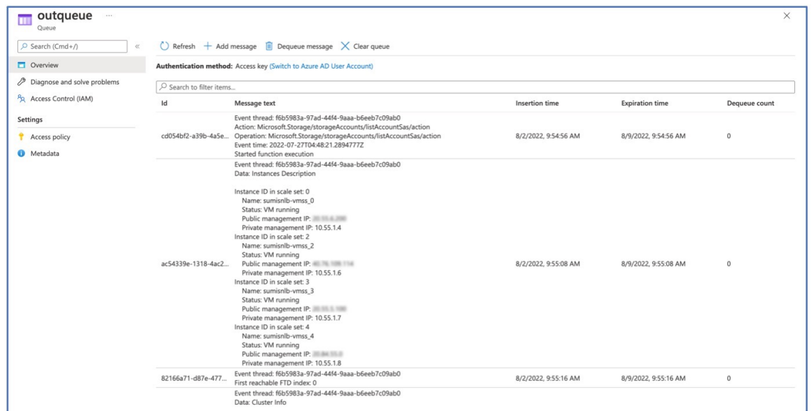
Figure 13: Outqueue
