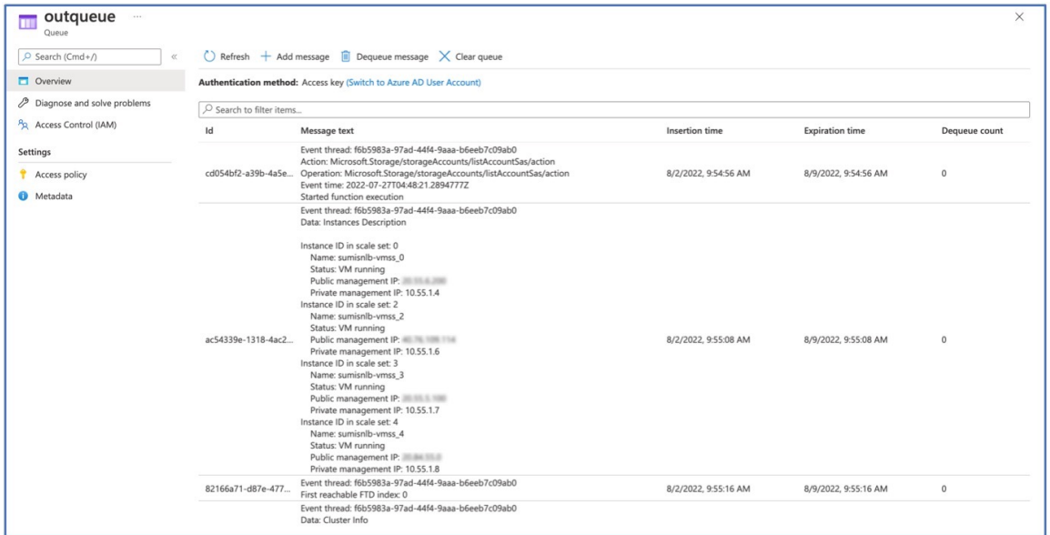
Figure 13: Outqueue
