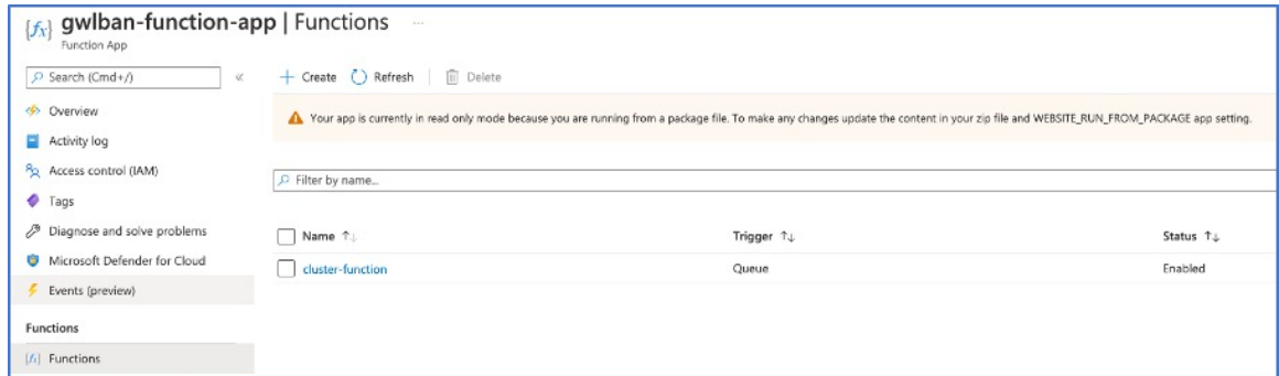
Figure 12: Queues
