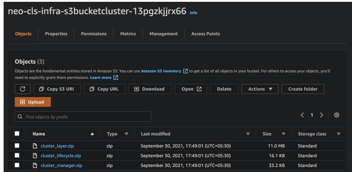
Figure 3: S3 Bucket
