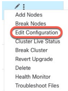
Figure 22: Edit Configuration
