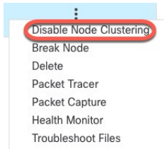
Figure 20: Disable Clustering
