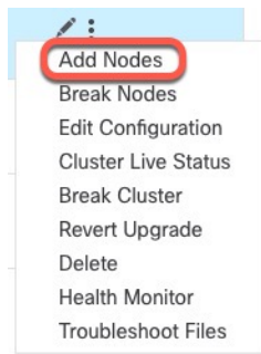
Figure 13: Add Nodes
