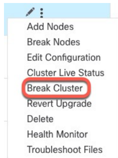
Figure 18: Break Cluster
