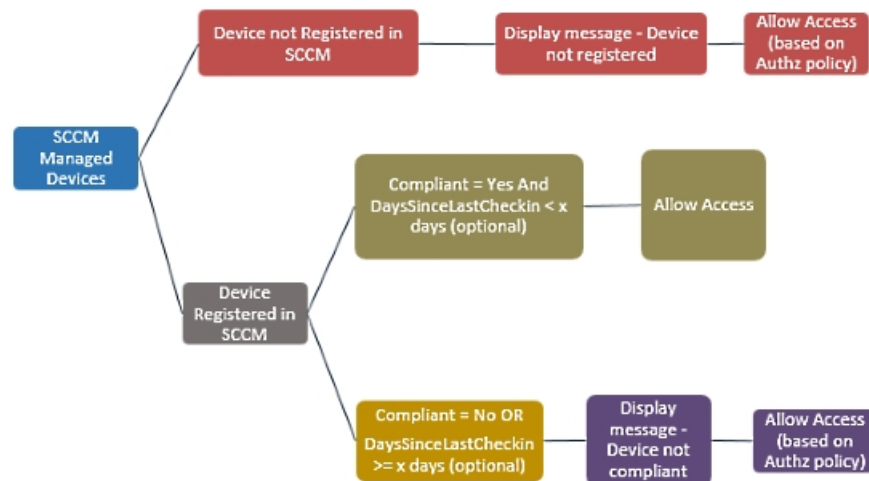
Figure 39: SCCM Workflow
