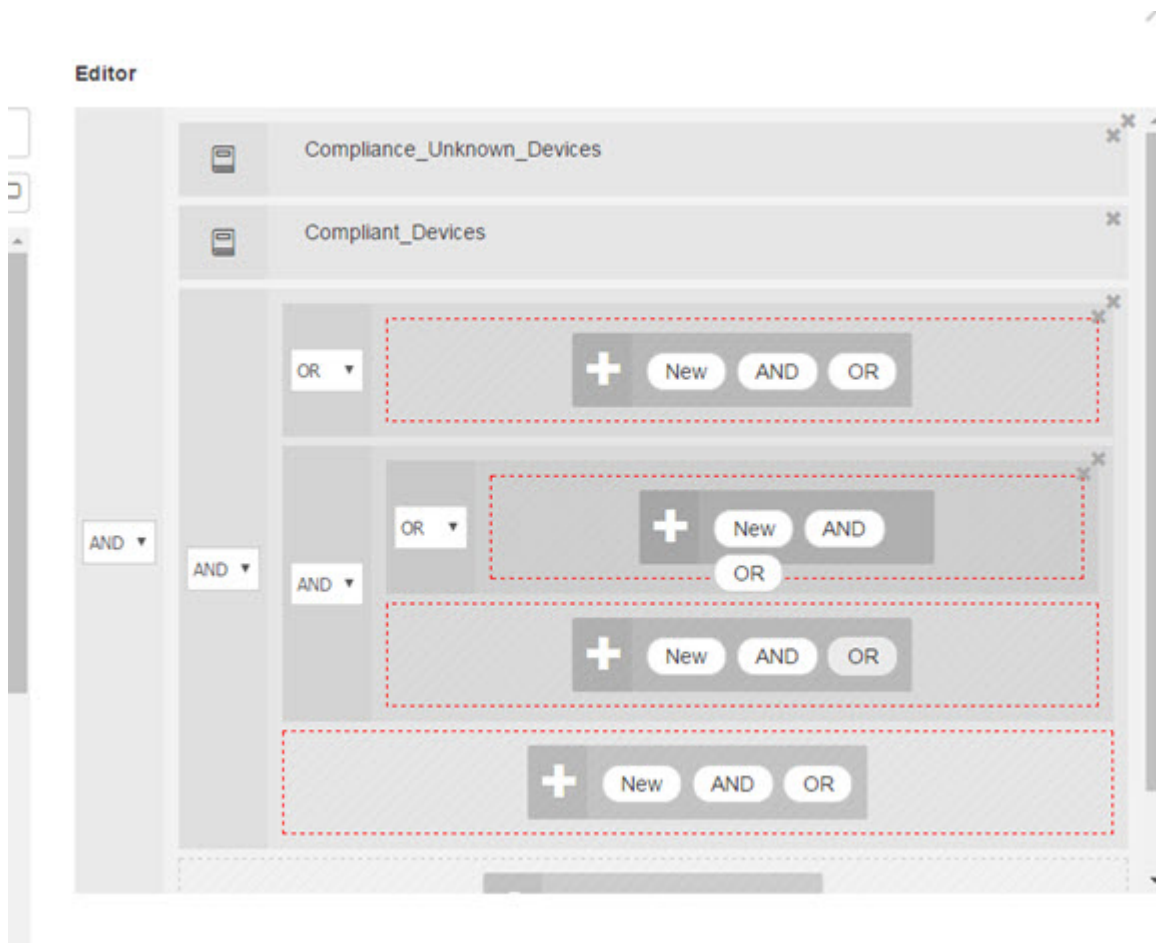
Figure 59: Editor—Conditions Hierarchy
