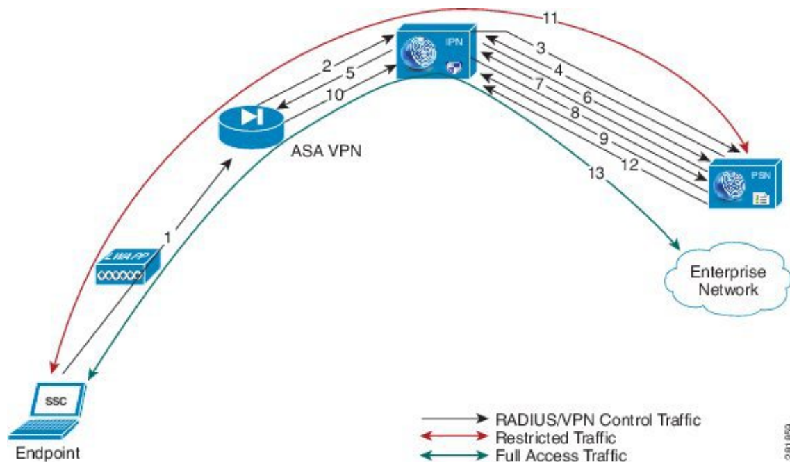
Figure 1: Inline Posture Policy Enforcement Flow
