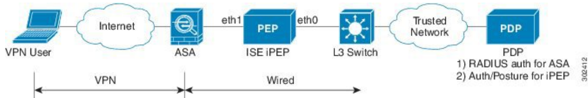
Figure 8: Cisco ISE Deployment with Inline Posture Node
