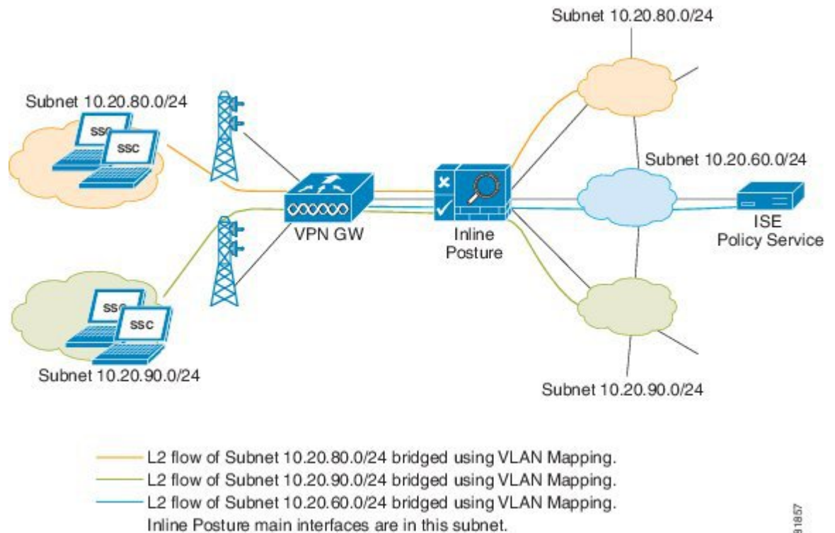
Figure 3: Inline Posture Bridged Mode Configuration
