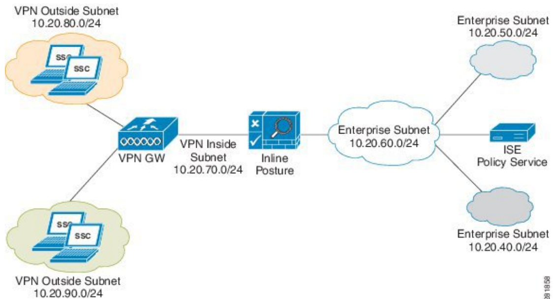
Figure 2: Inline Posture Routed Mode Configuration
