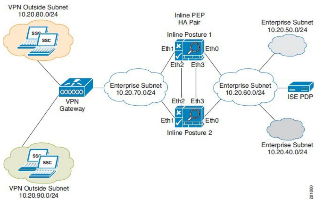
Figure 4: Inline Posture High-Availability Routed Mode Configuration
